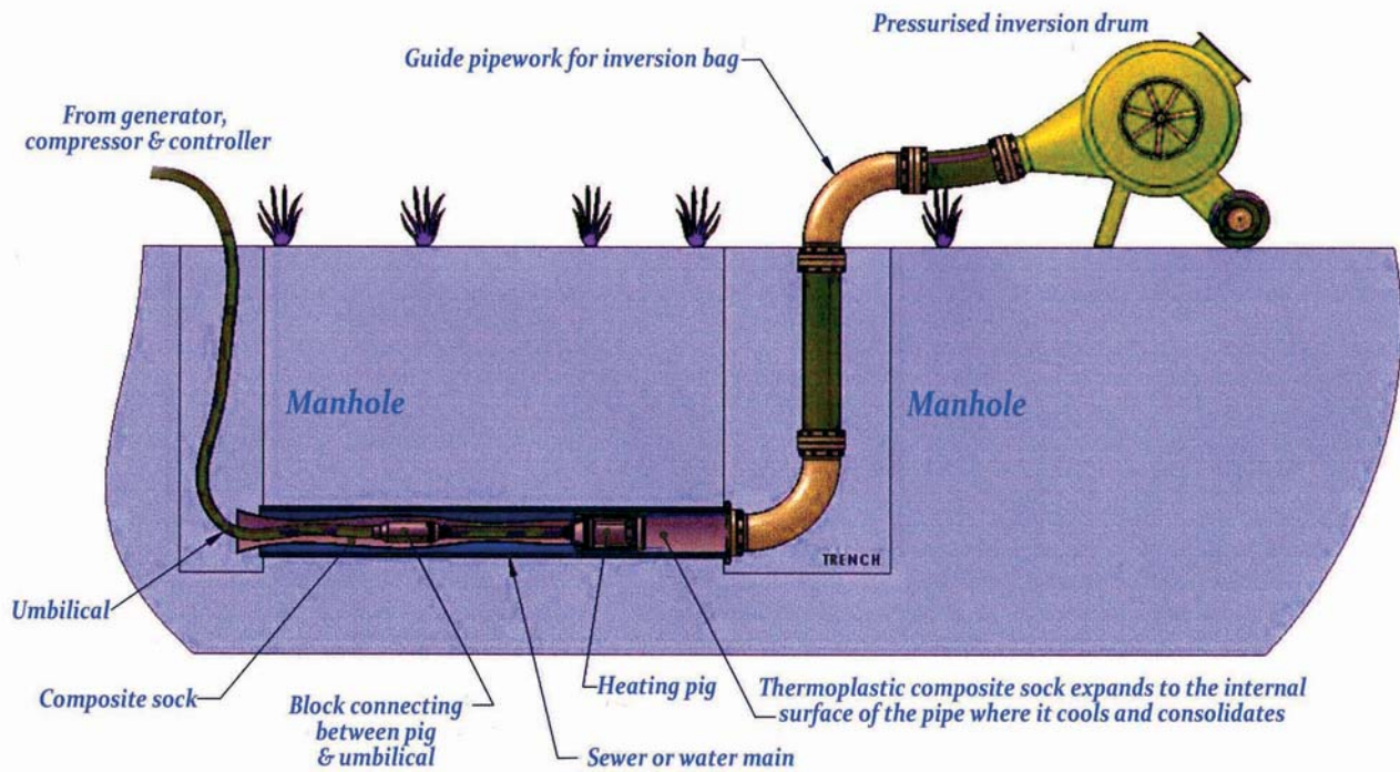
Schematic of the Aqualiner process
